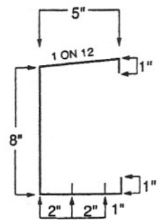
DOUBLE SLOPE
