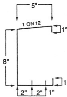
SINGLE SLOPE
